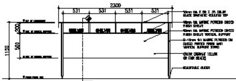
WRITING DECK FRONT ELEVATION SCALE: 1:30 METERS
